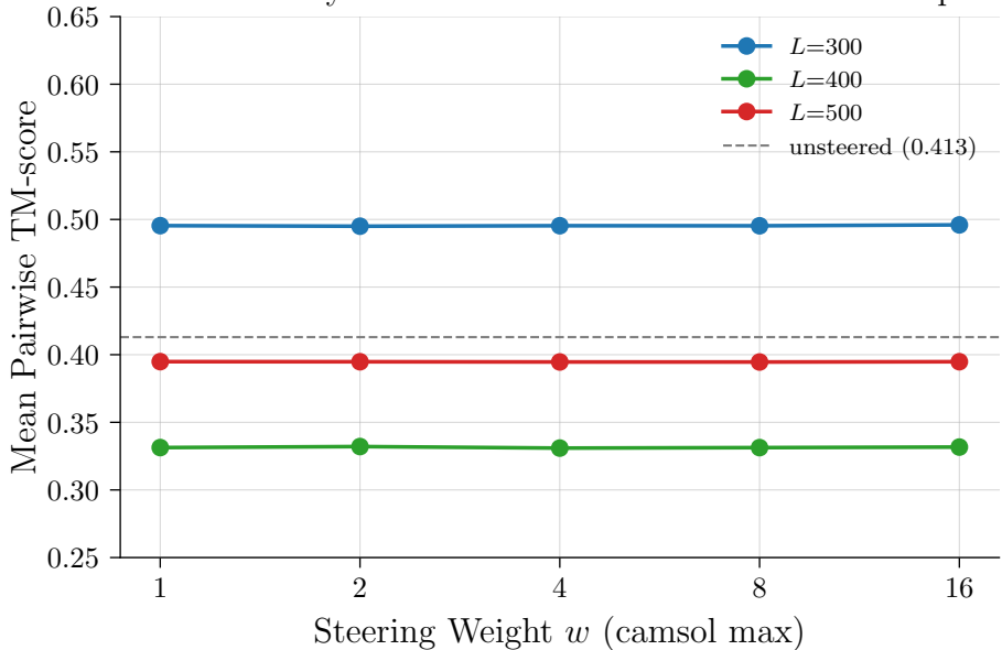
Mean TM Stays Flat Across w — Ensemble Not Collapsed
