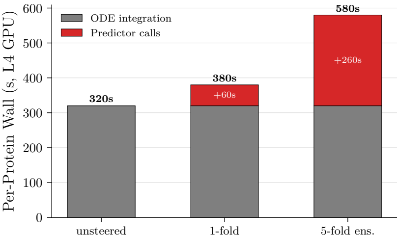
Walltime: Predictor Overhead Scales with Ensemble Size
