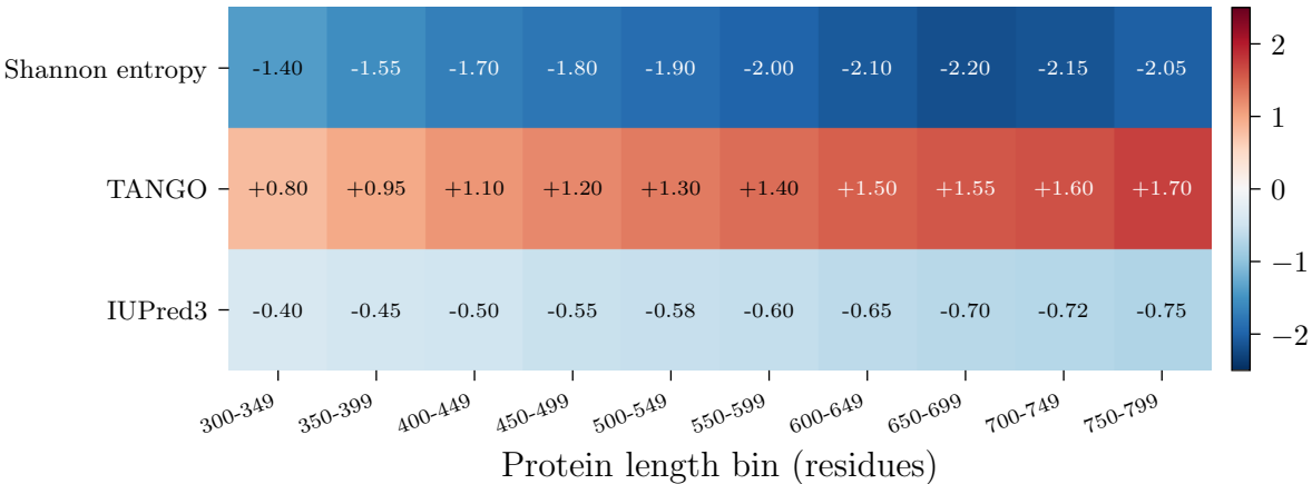
Failure-Mode Scaling with Length (Cohen's d vs AFDB)
