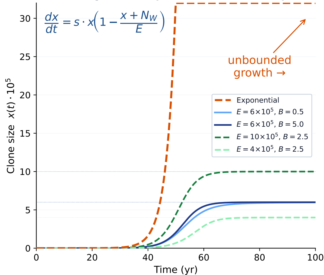
Mutant clone growth: displacement model vs exponential
