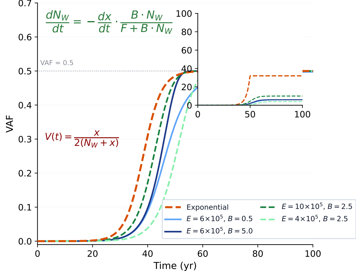
VAF dynamics: displacement model vs exponential ( s = 0.3 )
