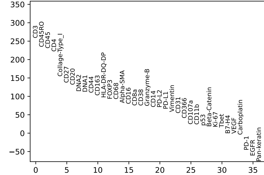
Cytotoxic T cell vs. rest
