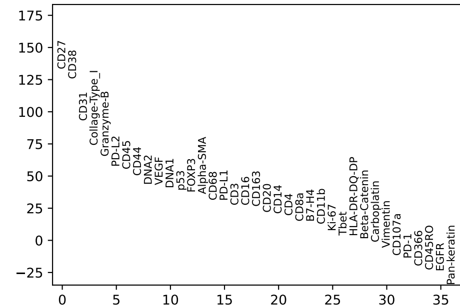
Reg T cell vs. rest
