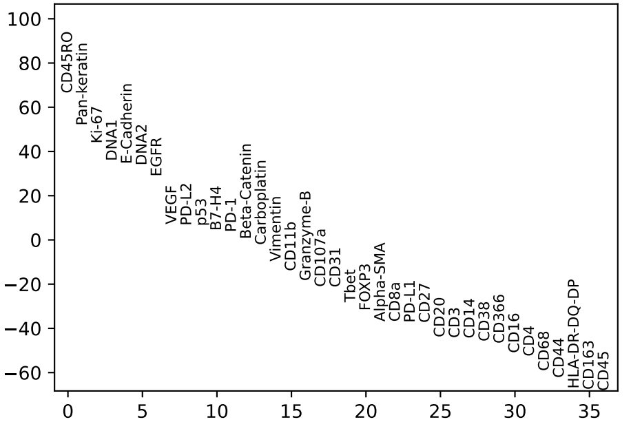
Immune/Cancer vs. rest
