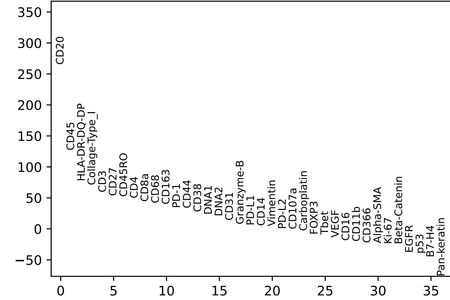
B-cell vs. rest
