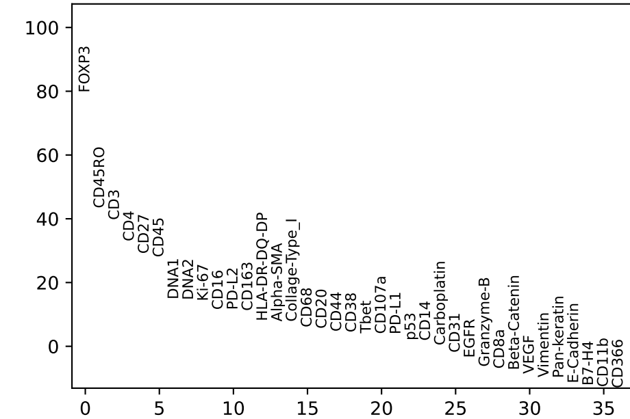
FOXP3+ Cancer vs. rest
