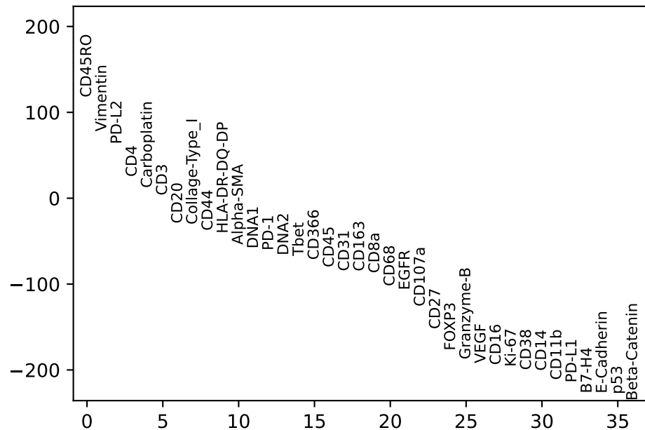
T-cell vs. rest
