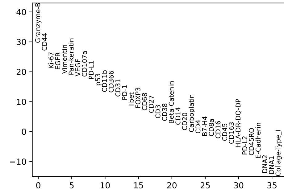
Vim+ Cancer / NK vs. rest
