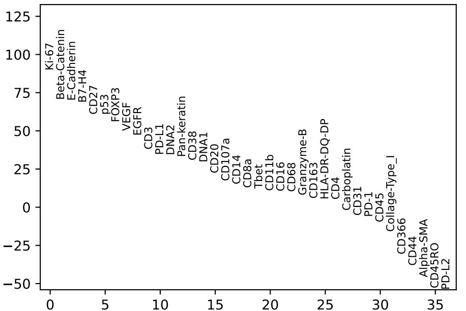
T-cell/Cancer vs. rest
