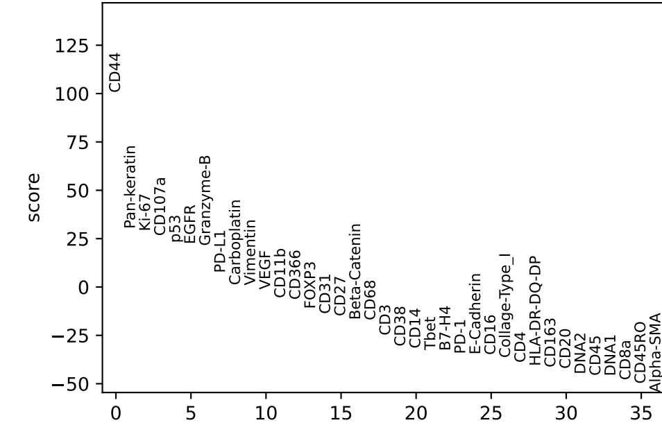
Cancer stem cell vs. rest
