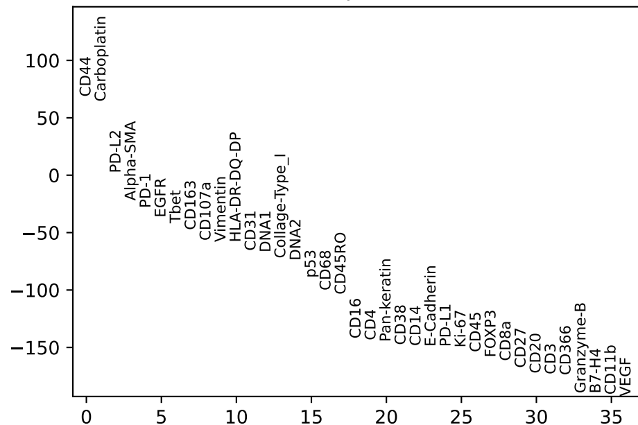
Th1 T helper vs. rest
