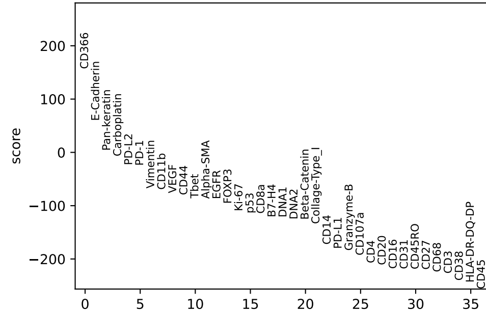
Exhausted T-cell vs. rest
