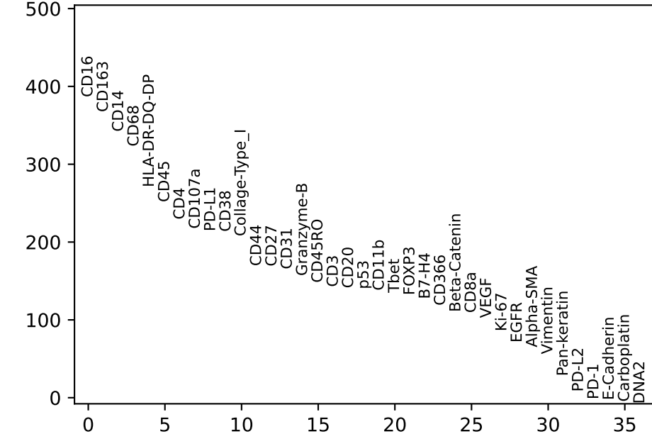
Monocytes vs. rest
