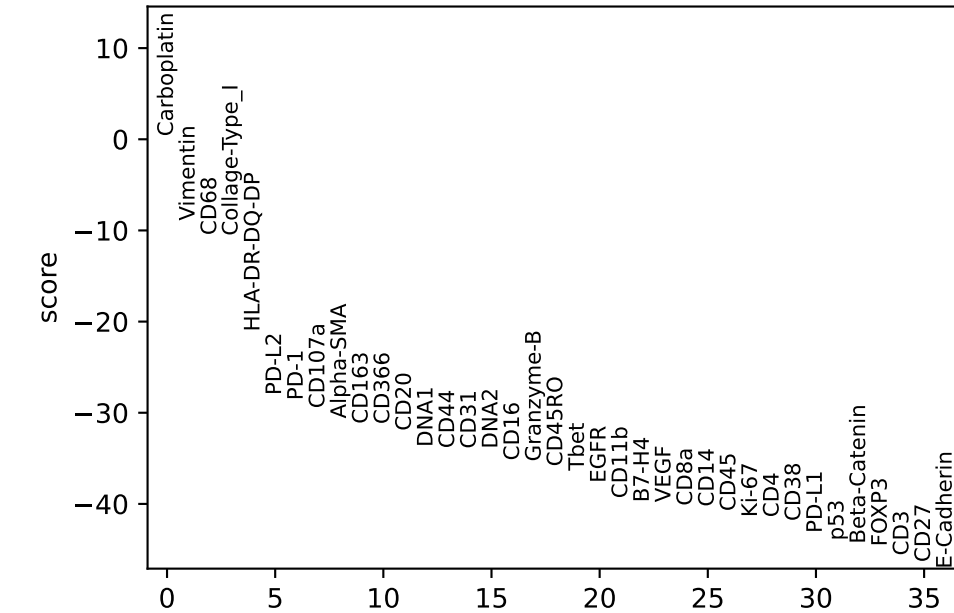
Macrophage vs. rest
