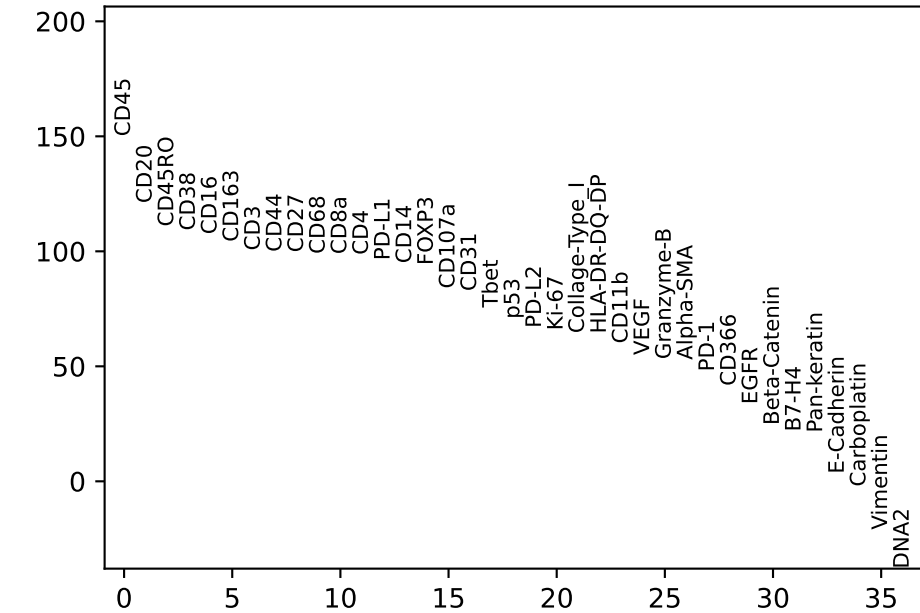
Memory T cell vs. rest
