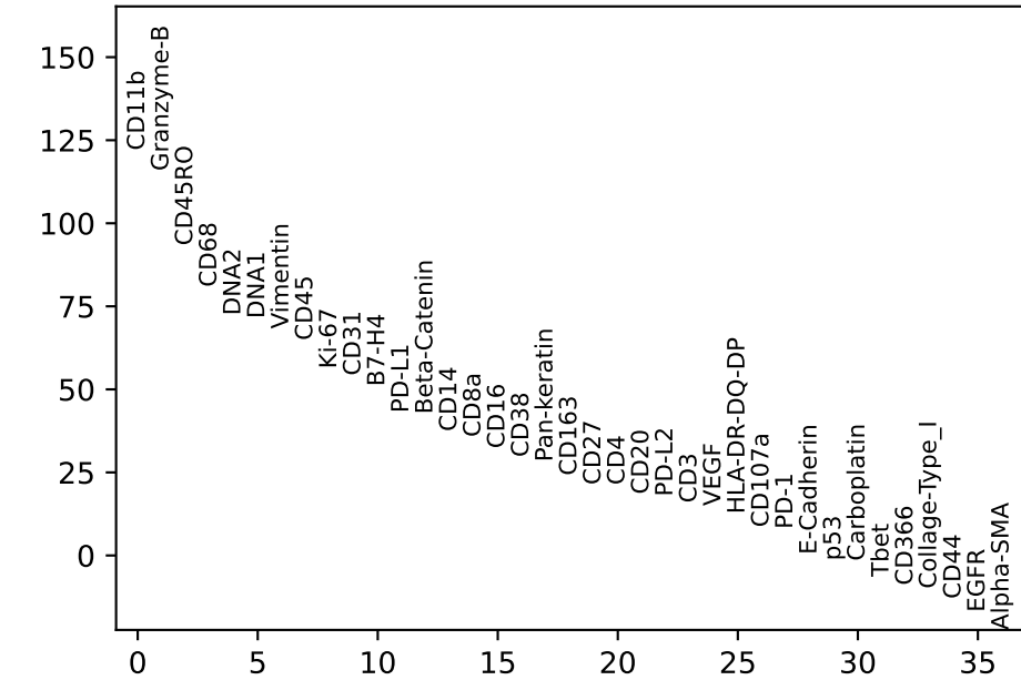
GB Active T cell vs. rest
