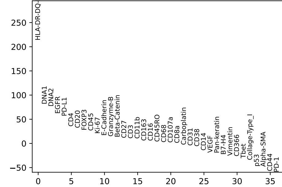
Antigen presenting cell vs. rest
