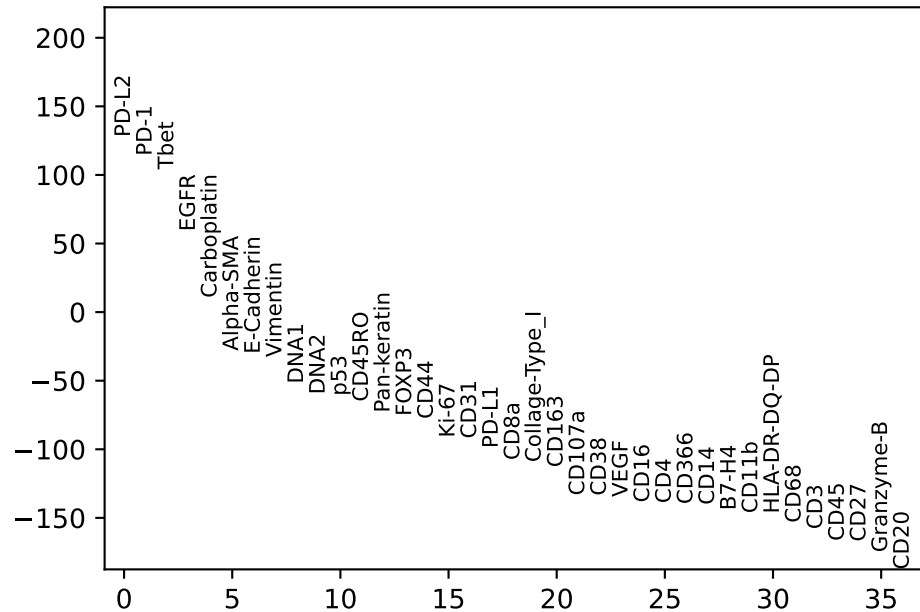
NK cell (FOXP3) vs. rest
