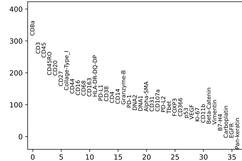
Mem CD8 T cell vs. rest
