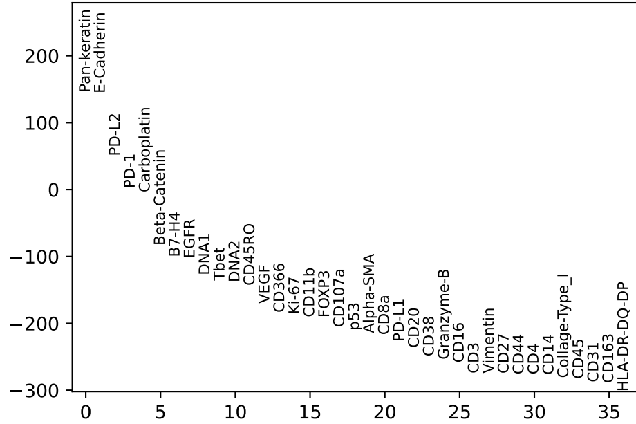
E-Cad cancer vs. rest
