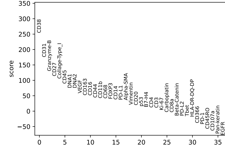
T/B cells vs. rest
