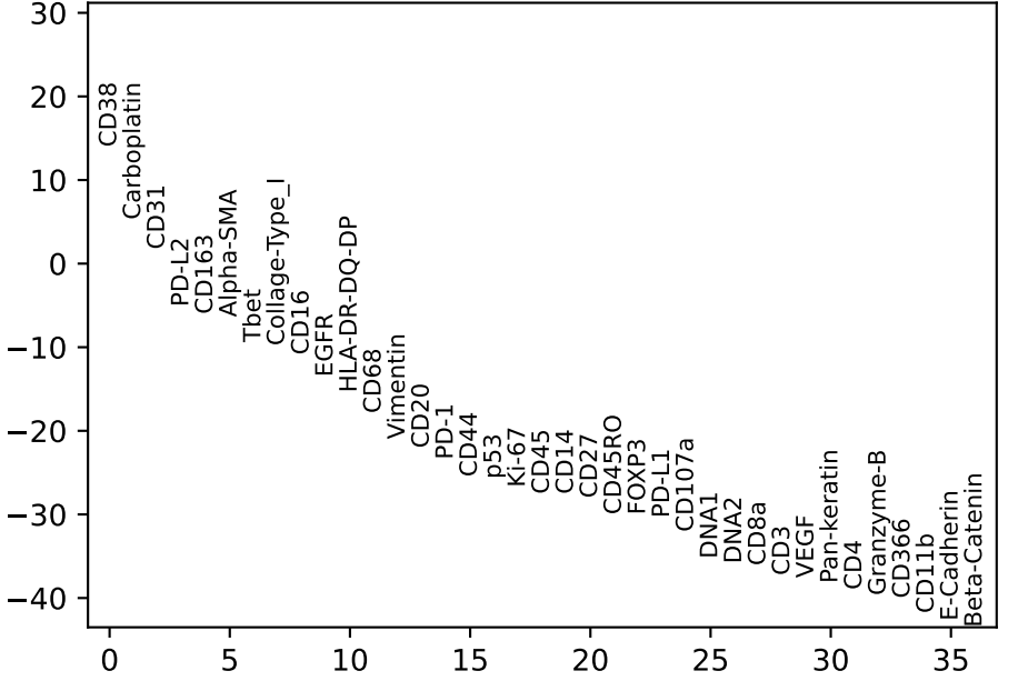
B/T/NK cell vs. rest
