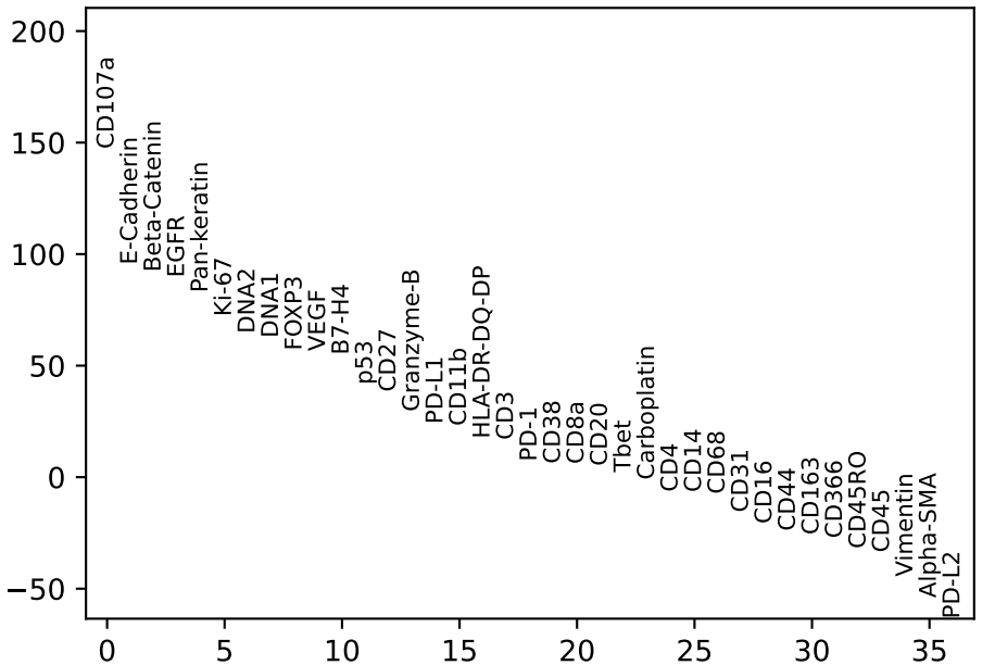
NK cells / Cancer vs. rest
