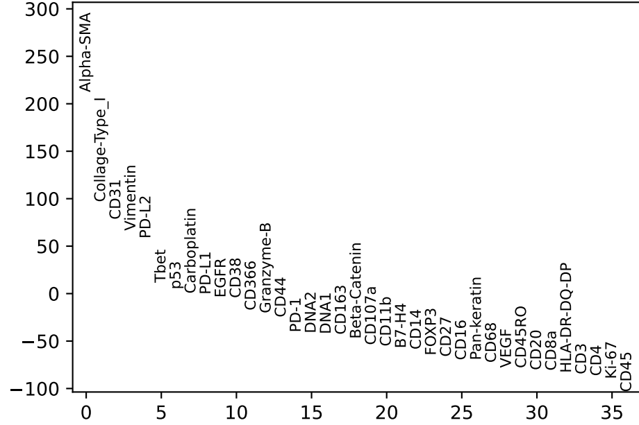
CAF vs. rest
