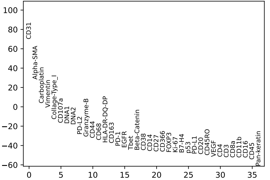
Endothelial vs. rest
