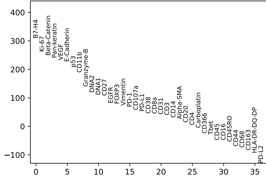
B7H4+ Cancer (CD11b) vs. rest
