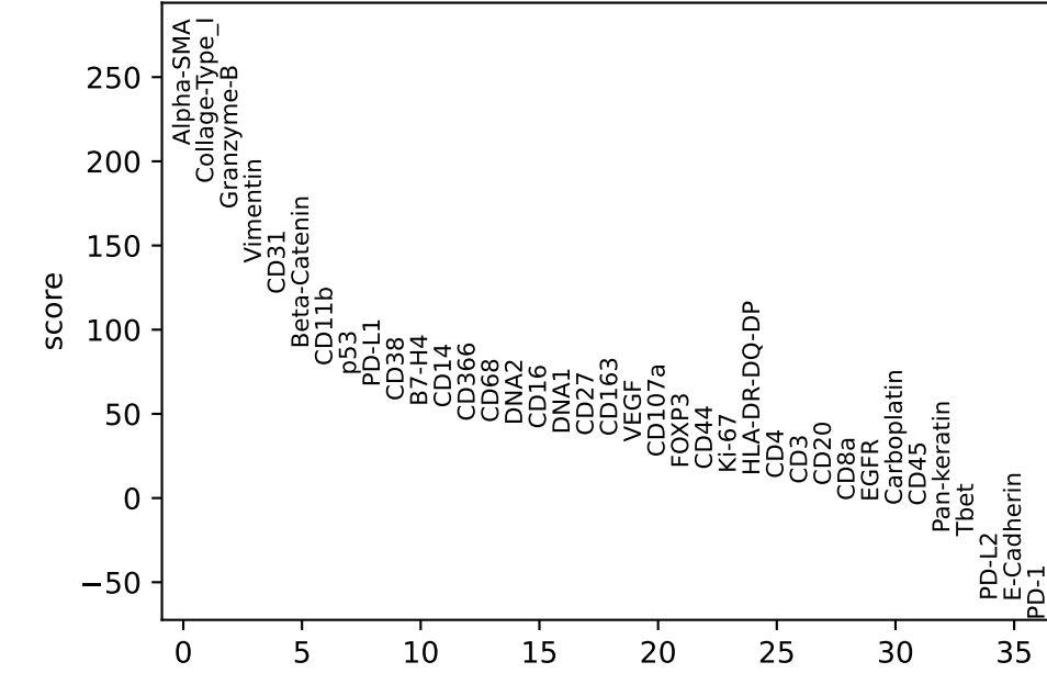
Alfa-SMA+ Monocytes vs. rest
