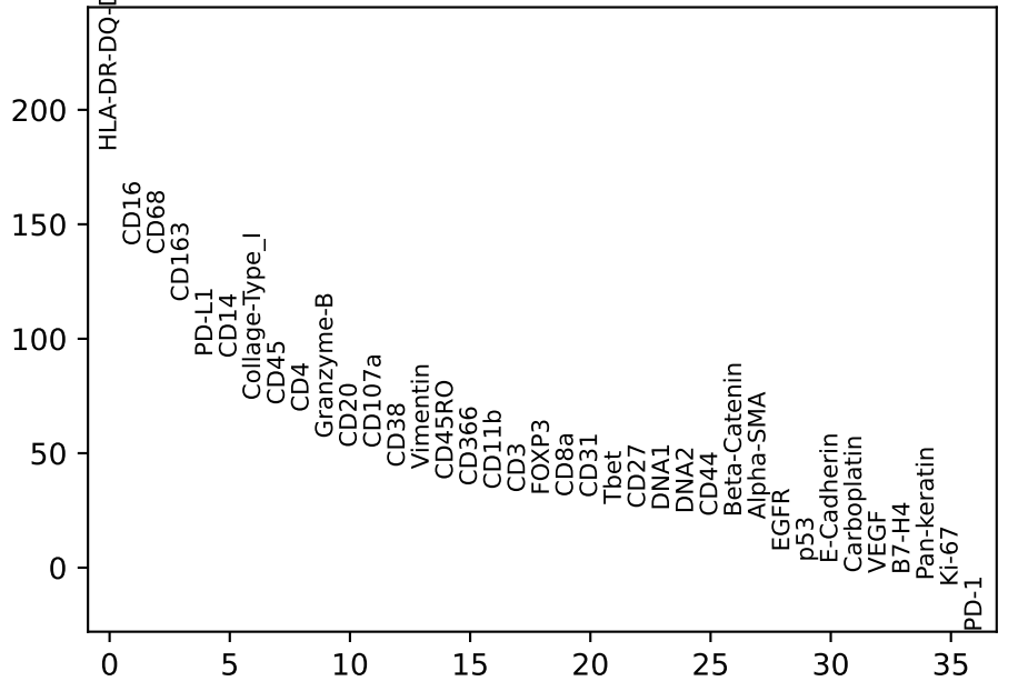
Monocyte (HLA) vs. rest
