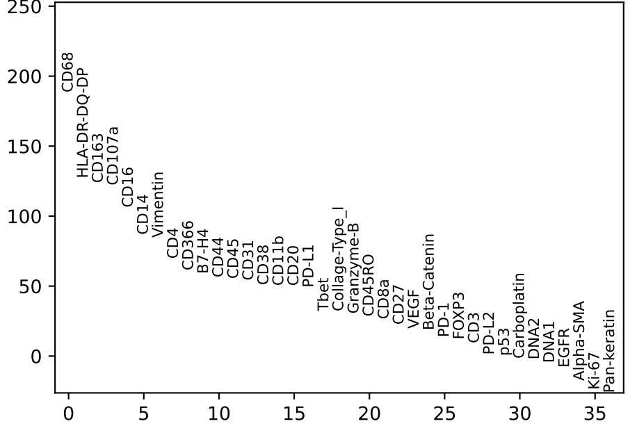
CD44+ MAC vs. rest
