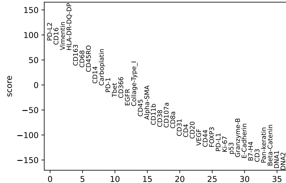
Monocyte (Tbet) vs. rest
