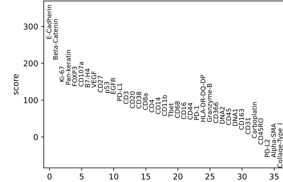
B7H4+ Cancer vs. rest
