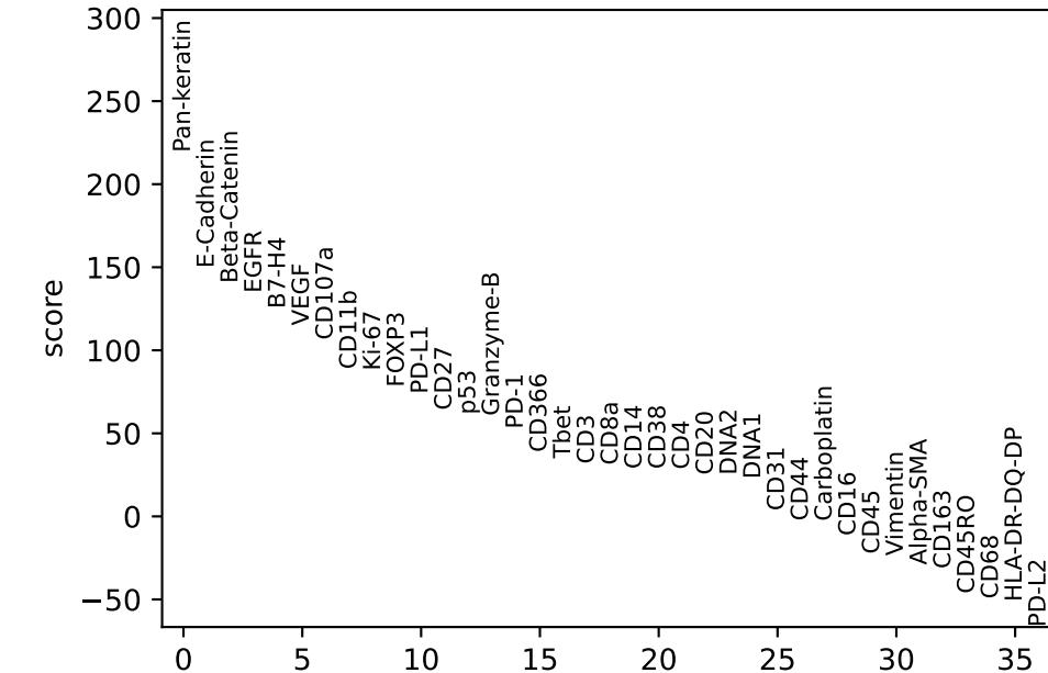
PanCK Cancer vs. rest
