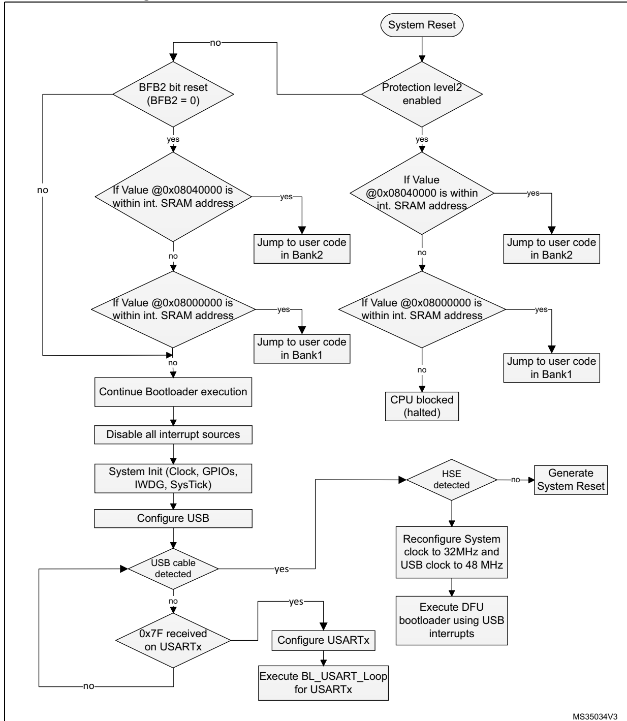
Figure 69. Bootloader selection for STM32L1xxxE devices
