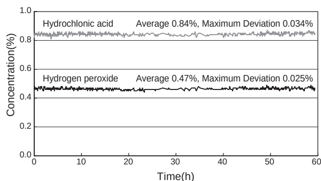
Fig.5 Stability of Measured Values (CS-152)
