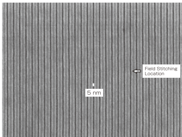
Field Stitching Pattern
