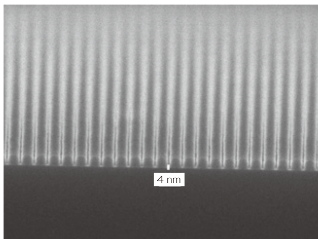
4 nm Line Pattern
