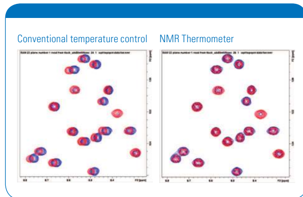
Fig. 7: Overlay of NOESY-HSQC (blue) and TOCSY-HSQC (red) experiments. Conventional temperature control results in peak shifts (left) induced by RF heating, NMR Thermometer control (right) maintains perfect chemical shift match between the spectra.
