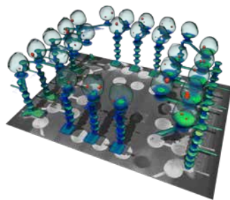
Ball grid array showing solder porosity. Imaged with micro-CT. Image courtesy of nanoX Technology Pte. LLtd.
