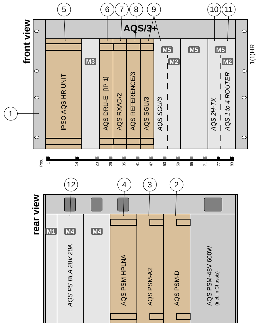
Figure 6.2 AQS/3+ for 2 channel AVANCE III HD (internal IPSO)
