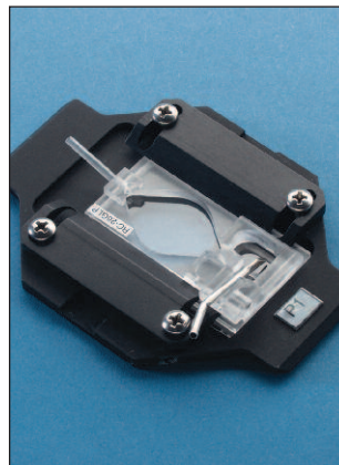
RC-26GLP shown in a P-1 chamber platform
