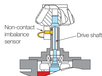
Non-contact imbalance protection
