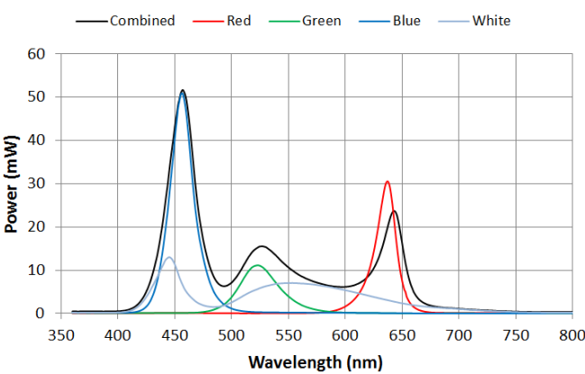
RGBW Optical Spectrum
