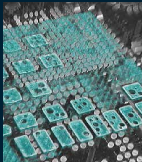
Computed Laminography of PCB, Clipping Plane
