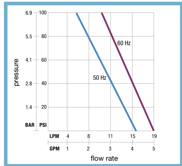
Pumping Capacity for TI Pump
