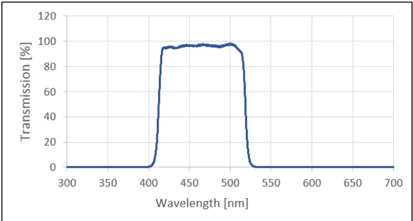
Figure 19: Transmission spectrum of filter 'Blue2 NB'
