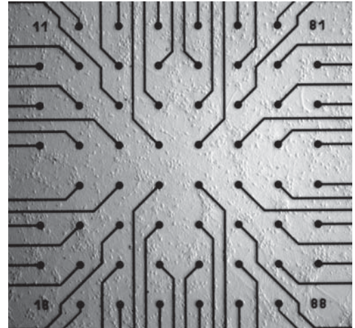
Standard electrode layout grid 8 x 8
