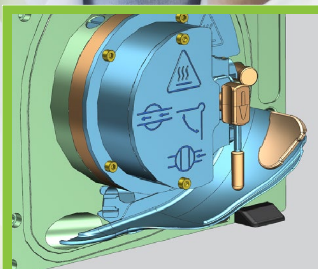
New source shield technology featured in the Xevo TQ Absolute Mass Spectrometer minimizes contamination and increases uptime.
