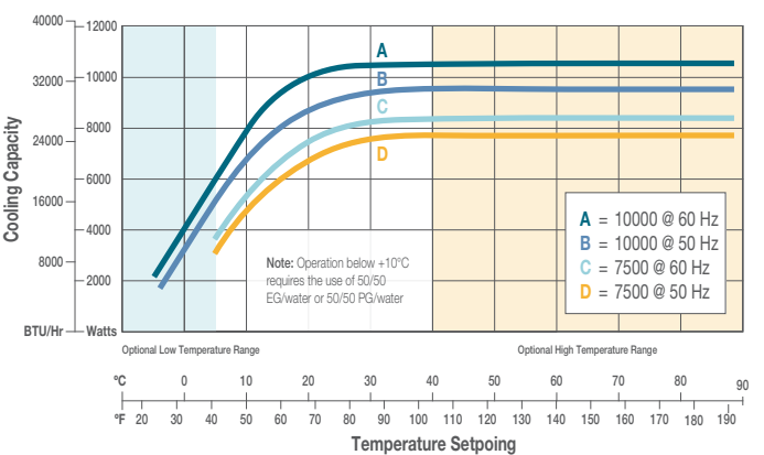
ThermoFlex 7500 & 10000
