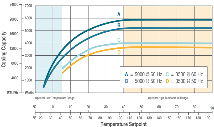
ThermoFlex 3500 & 5000
