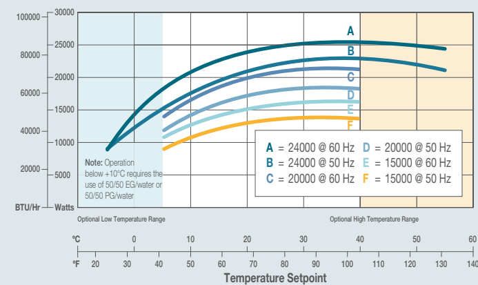
ThermoFlex 15000, 20000 & 24000
