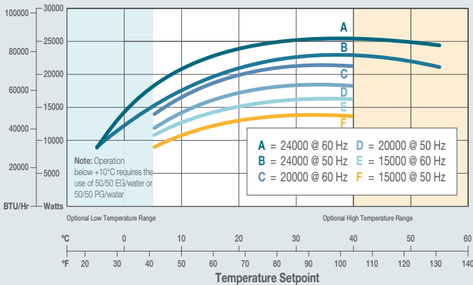
ThermoFlex 15000, 20000 & 24000
