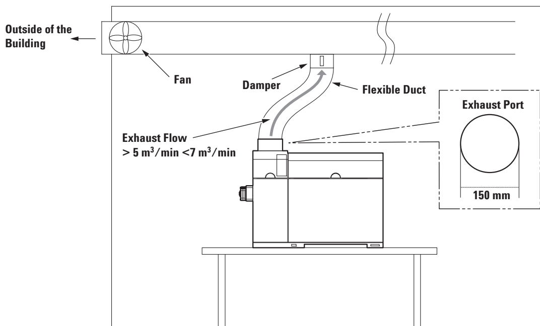
Figure 14 Exhaust Duct Connection
