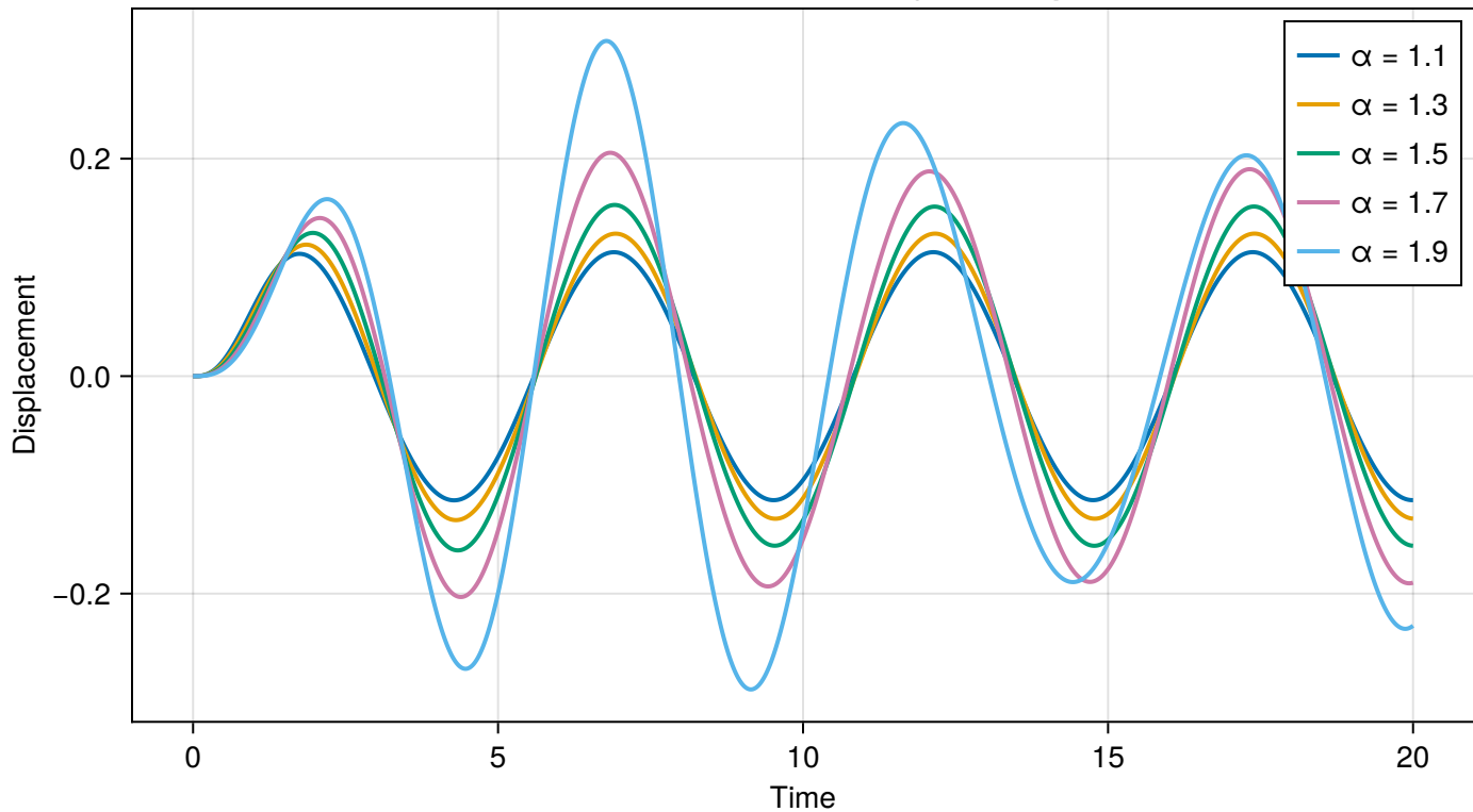
Effect of fractional order \alpha on system response
