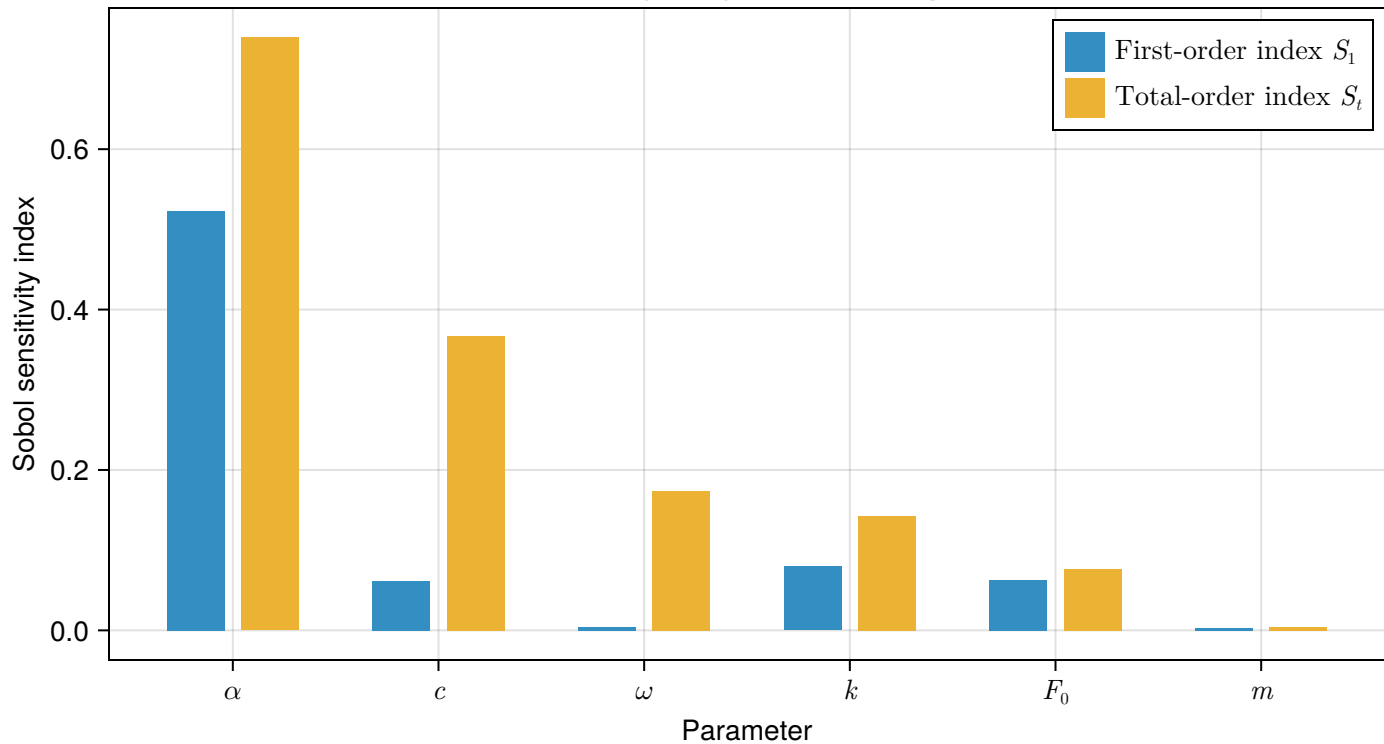
Global sensitivity analysis of RMS displacement
