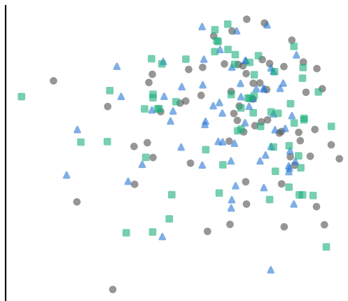
meander-oxbow
