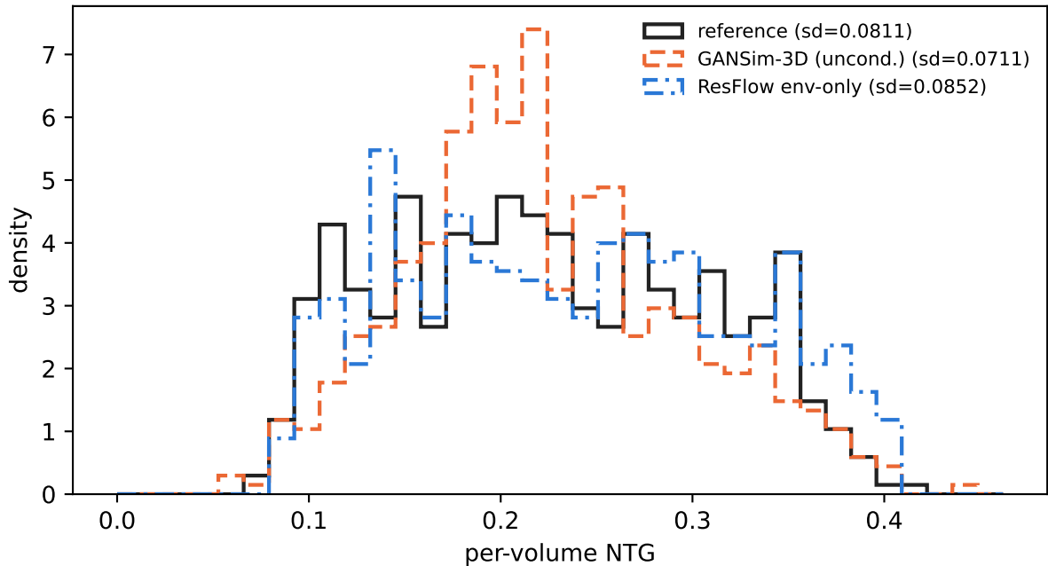
channel:PV_SHOESTRING: per-volume NTG spread (512 volumes each)
