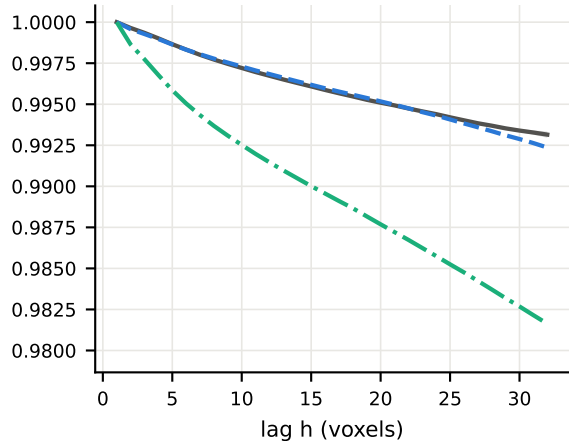
meander-oxbow — x
