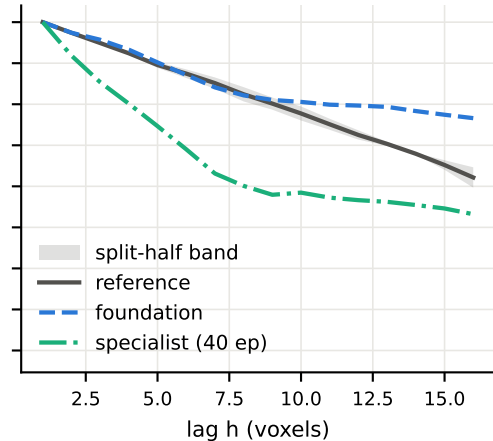
meander-oxbow — z
