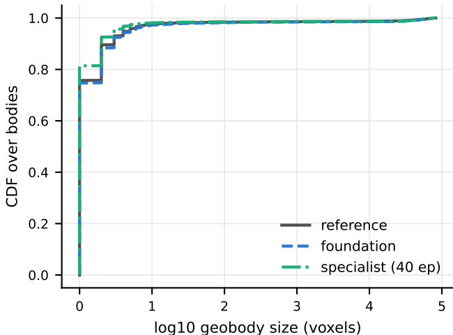
CB labyrinth — geobody sizes
