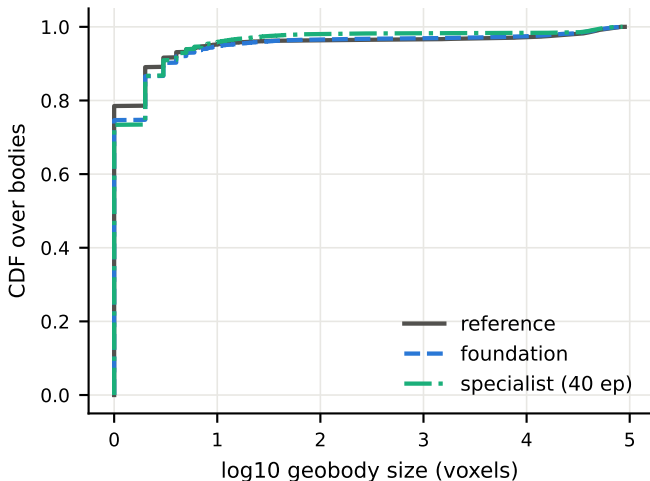
delta — geobody sizes
