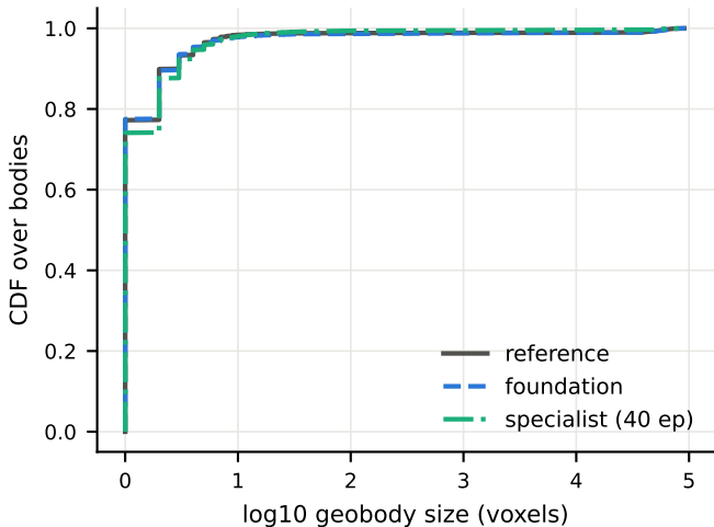
meander-oxbow — geobody sizes
