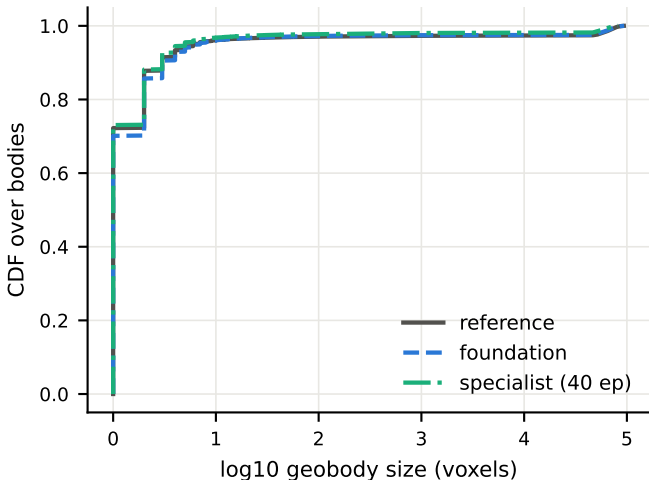
SH proximal — geobody sizes
