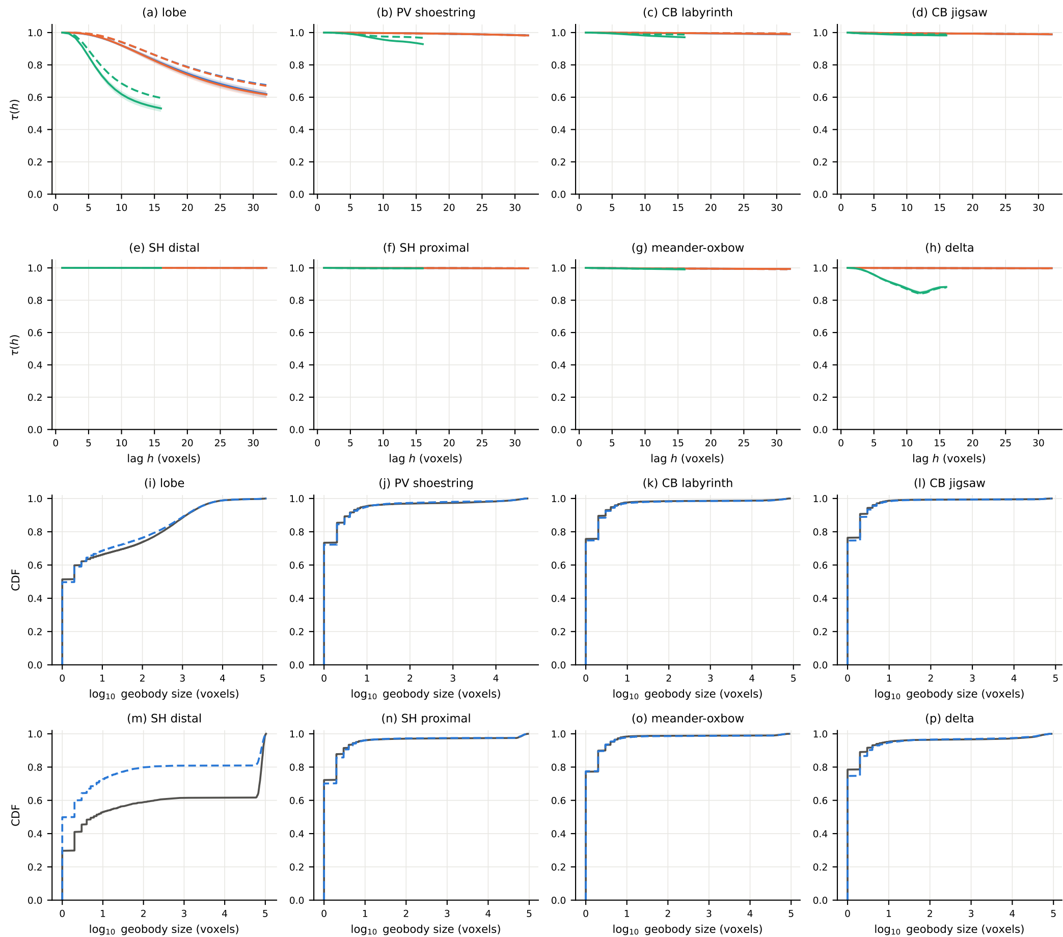
Connectivity functions (top) and geobody-size CDFs (bottom)
