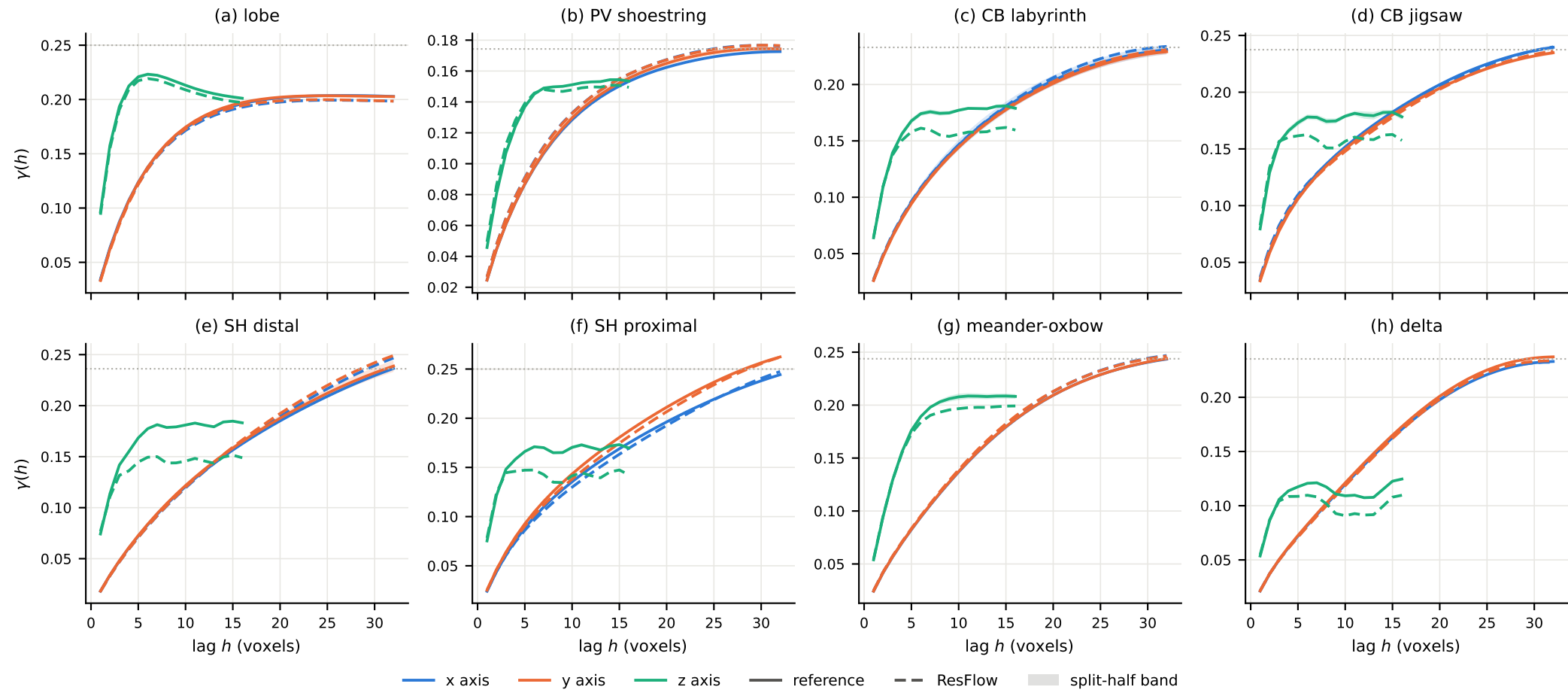
Indicator variograms: reference vs ResFlow (dotted: sill p(1 - p) )
