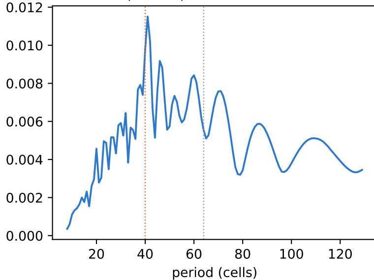
mean profile spectrum (dotted: 40, 64)
