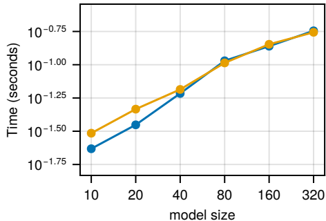
Code generation
