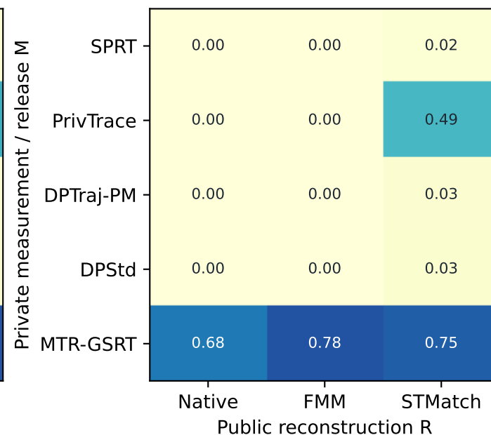
Road continuation MRR
