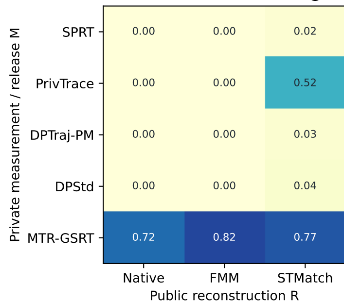
Road continuation Hit@1
