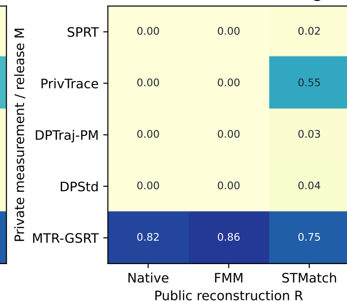
Route retrieval NDCG@5
