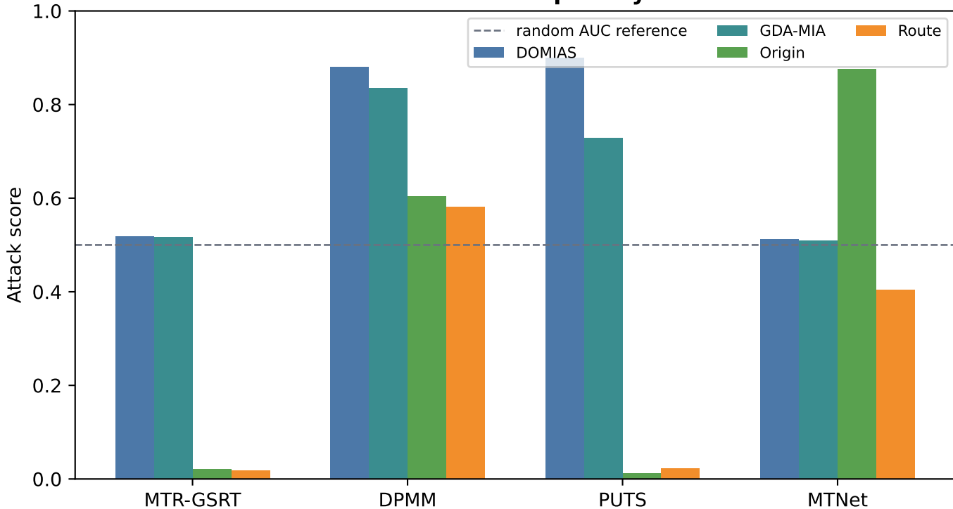
Published-interface privacy audits
