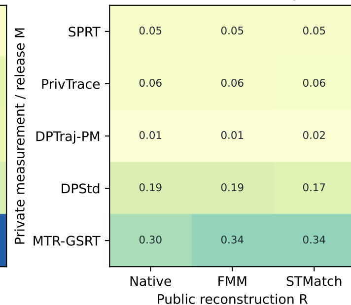
Route retrieval NDCG@5
