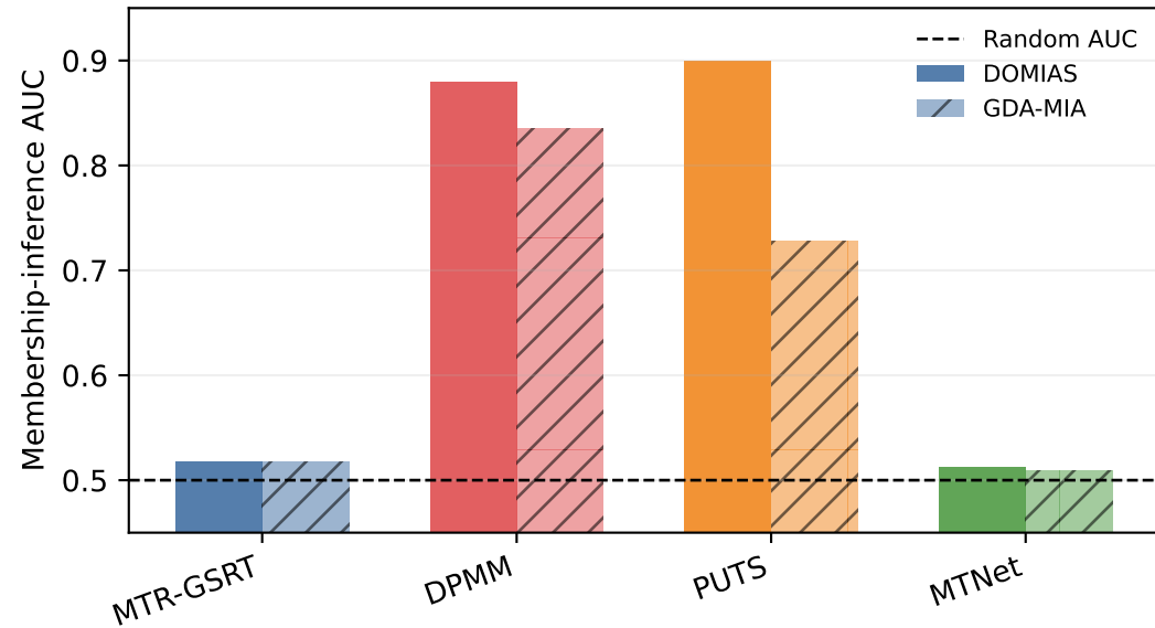
Population membership inference
