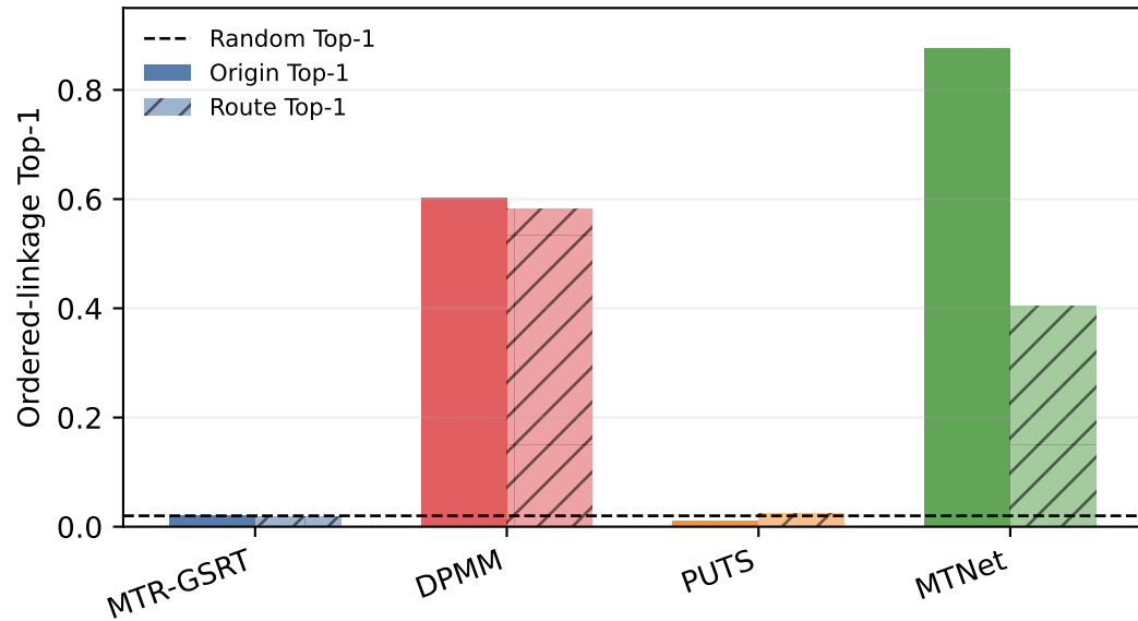
Input-output correspondence attack
