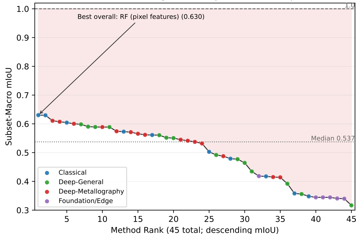
Global Ranking: No Family Closes the Gap
