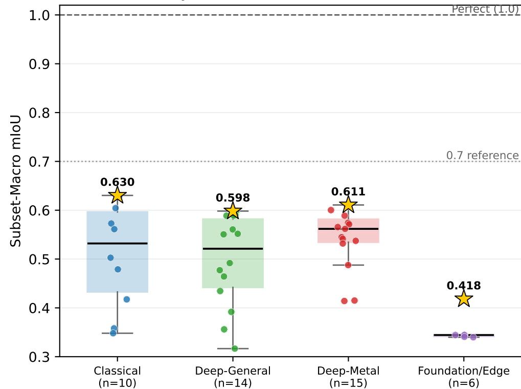
Family-Wise Performance Distribution
