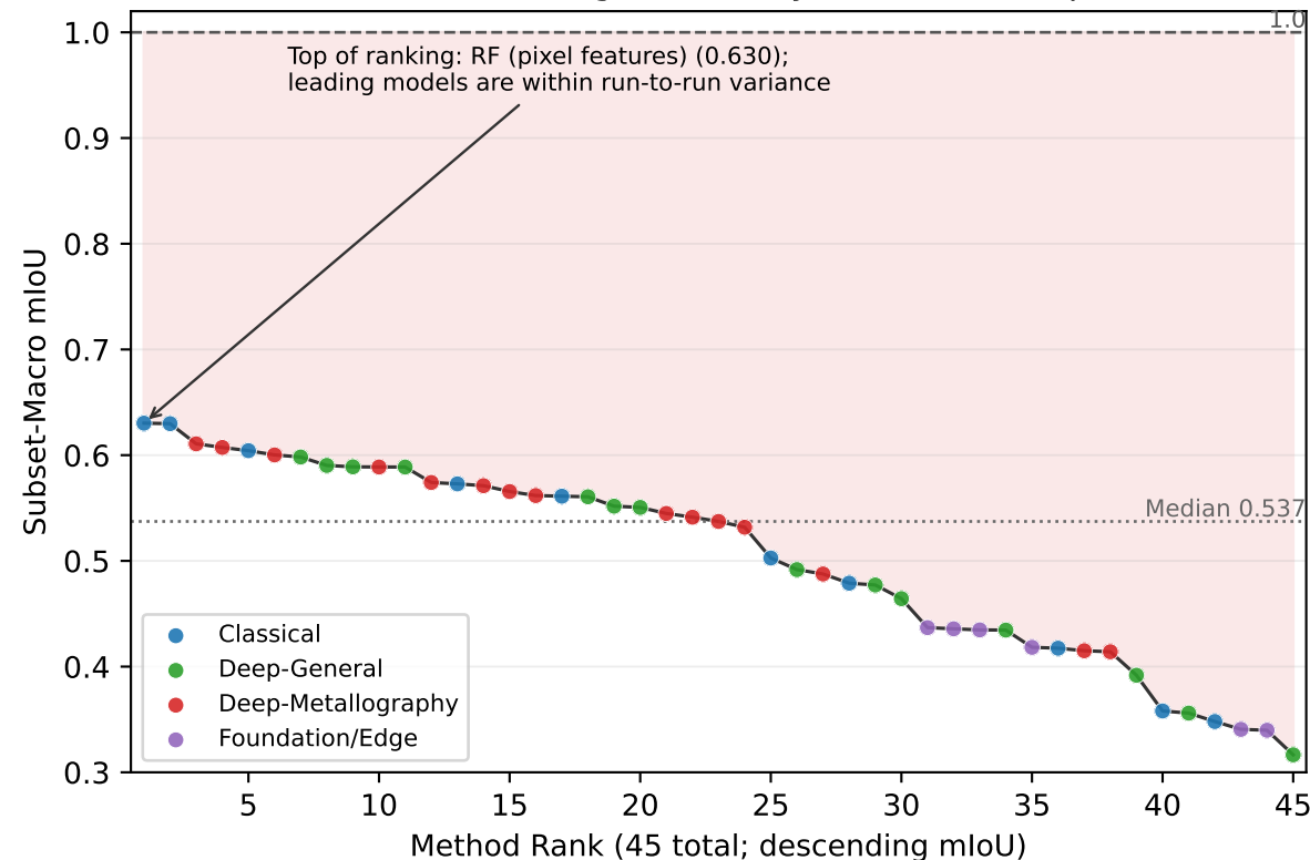
Global Ranking: No Family Closes the Gap
