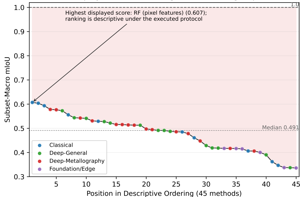
Displayed Score Ordering and Remaining Gap
