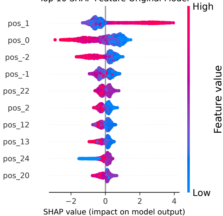
Top 10 SHAP Feature Original Model
