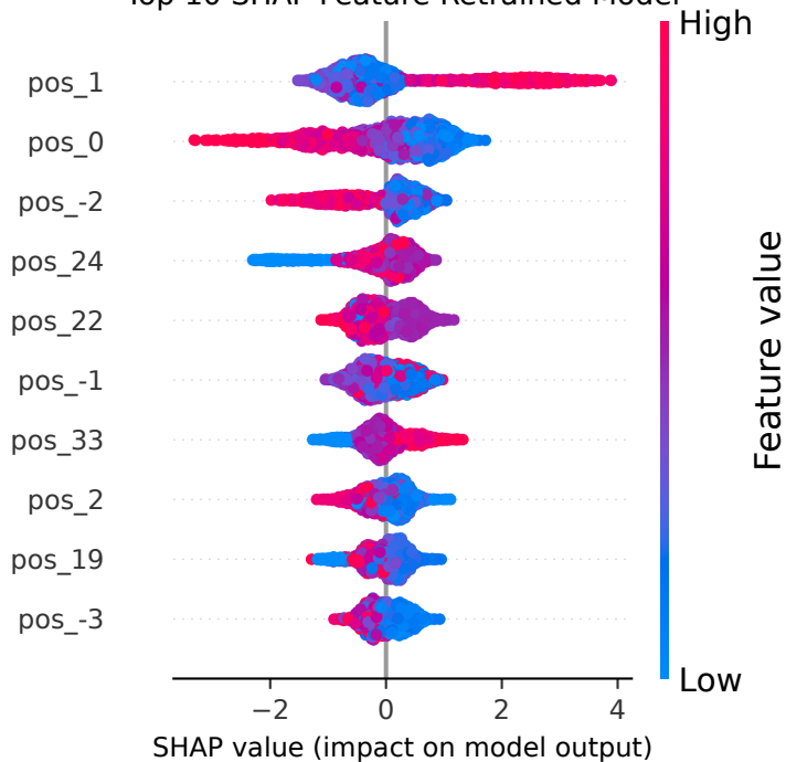
Top 10 SHAP Feature Retrained Model
