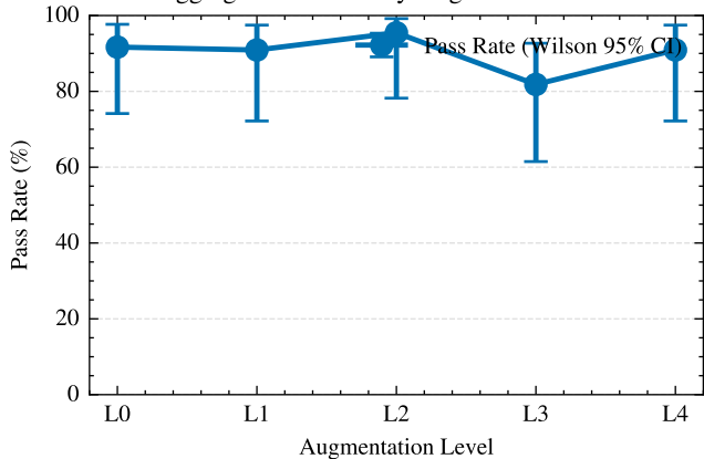
Aggregate Pass Rate by Augmentation Level
