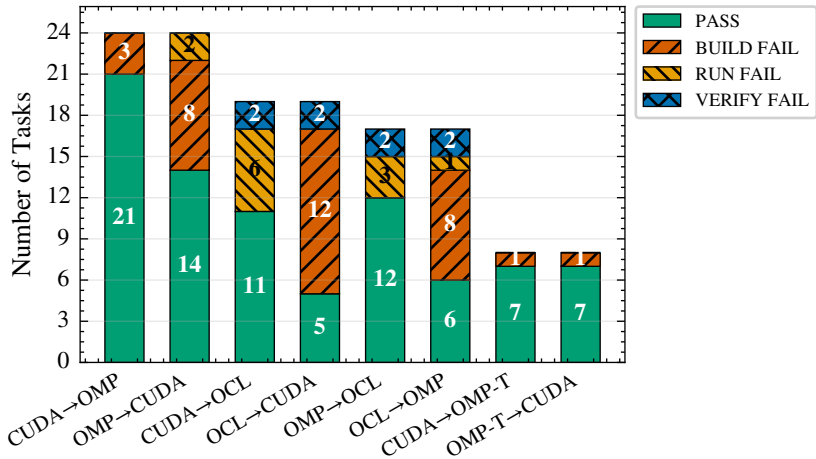
Failure Taxonomy: Status Distribution by Direction (L0, All Suites, Azure GPT-5.4)
