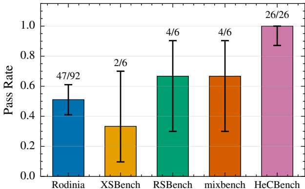
L0 Pass Rate by Suite (Azure GPT-5.3-codex)
