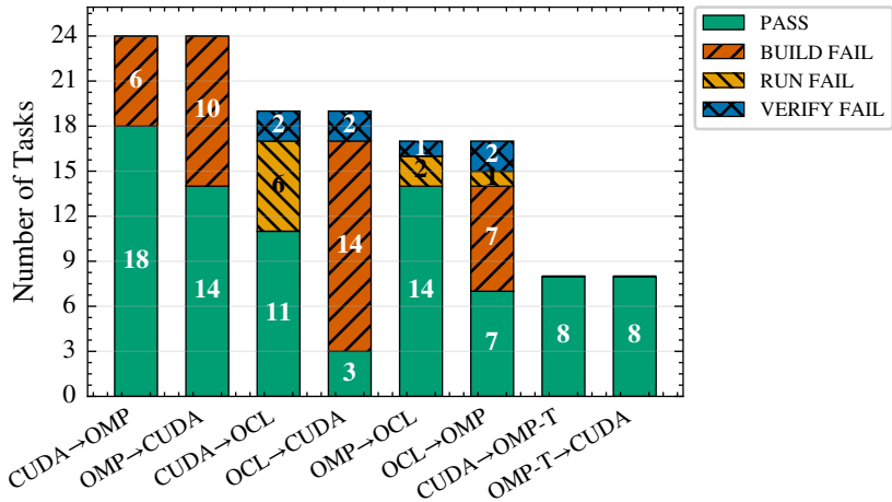
Failure Taxonomy: Status Distribution by Direction (L0, All Suites, Azure GPT-5.3-codex)
