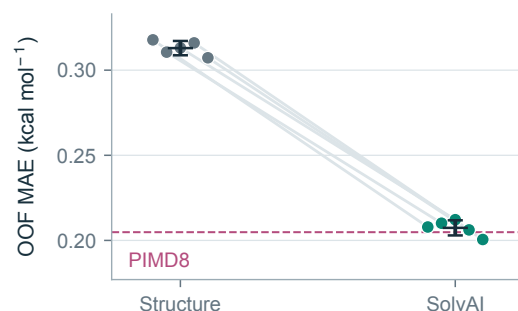
Figure 4: Molecule-aligned response descriptors improve a matched hydration endpoint. a , The matched control removes the responses; the shuffled control reassigns the complete response block among molecules. Labels, structural descriptors, architecture, weights, folds and seeds are fixed. The assignment sketches are illustrative; shuffled MAE is the mean of five permutations. b , Fixed-partition progression adds eight COSMOtherm, Abraham and corrected-solvent descriptors, then SMD(water), then six ConfSolv summaries. The dashed magenta line marks ARROW/PIMD8 on the same 85 solutes, as an accuracy reference rather than an input or training source. c , Paired absolute errors in \text{kcal mol}^{-1} for every molecule. Shading marks lower error with responses. d , MAE change for predeclared response blocks relative to structure only; bars are 95% molecule-bootstrap intervals from 100,000 resamples. e , Paired results for five complete split repeats. Thin lines join methods within the same partition; black marks show mean \pm sample s.d.
